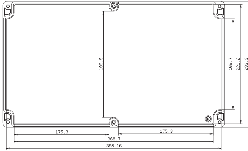
Kapak / Cover
