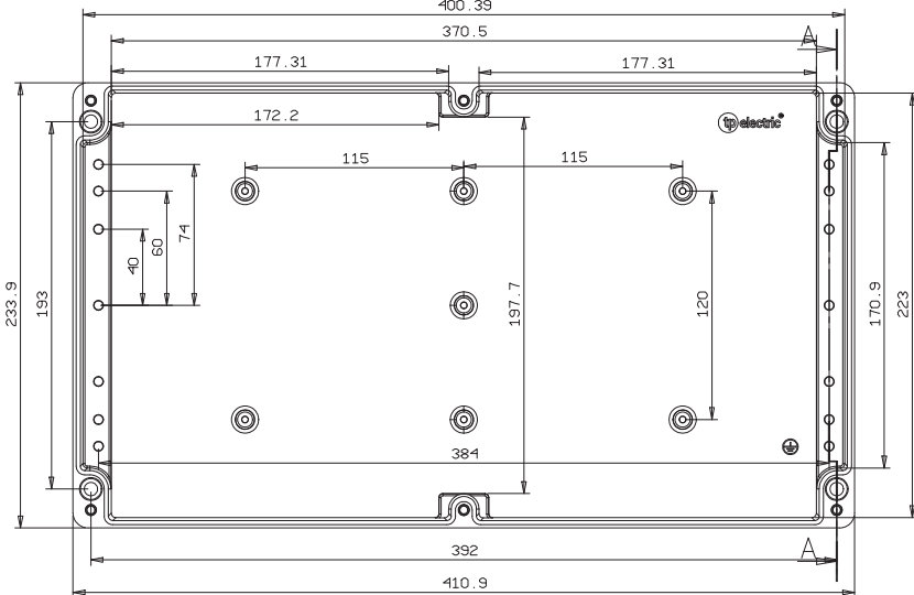
Gövde / Housing
