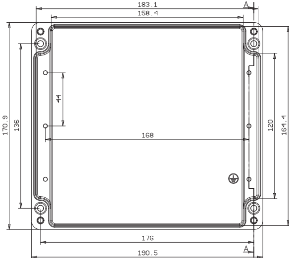
Gövde / Housing
