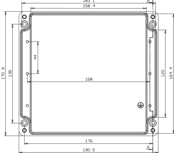
Gövde / Housing
