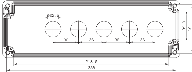
Kapak / Cover
