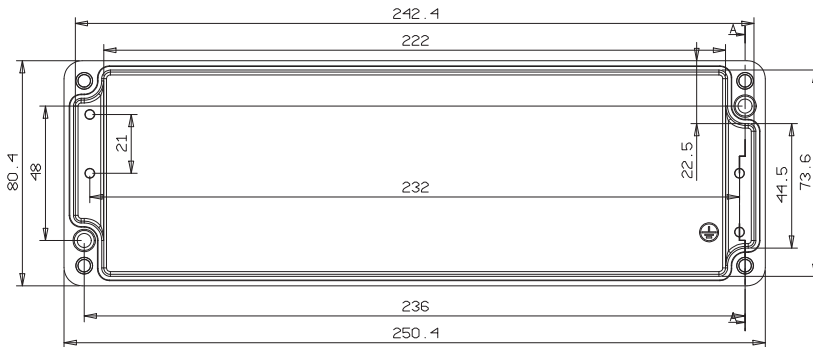
Gövde / Housing
