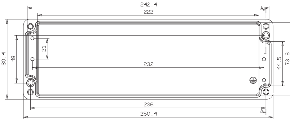
Gövde / Housing
