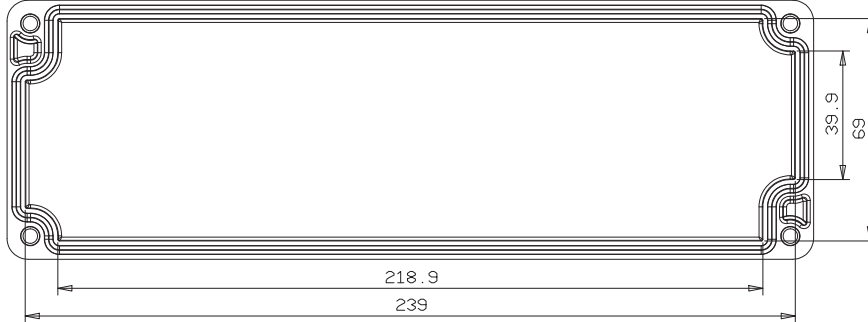
Kapak / Cover
