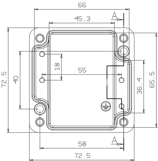
Gövde / Housing
