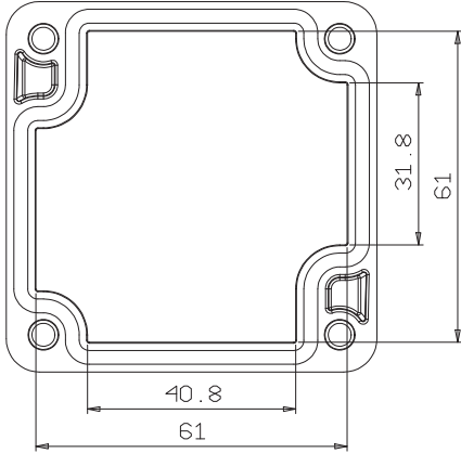
Kapak / Cover
